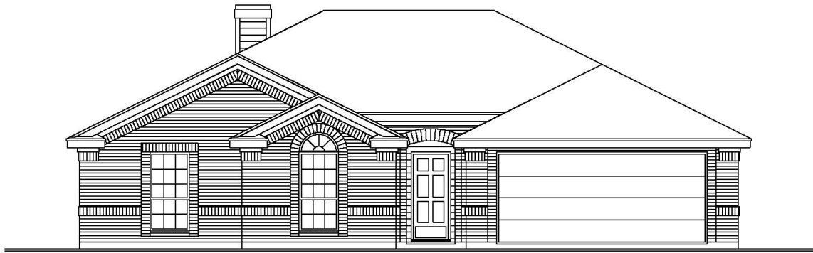
FRONT ELEVATION "A"
